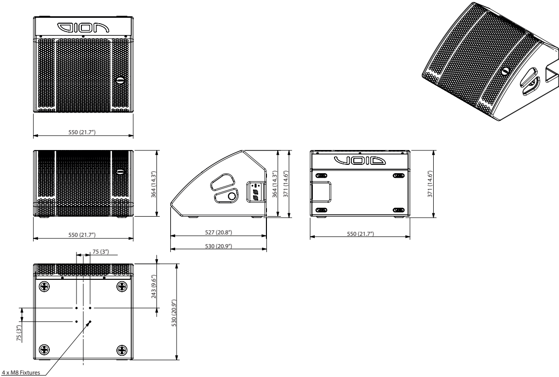
Figure 4.3: Dimensions
