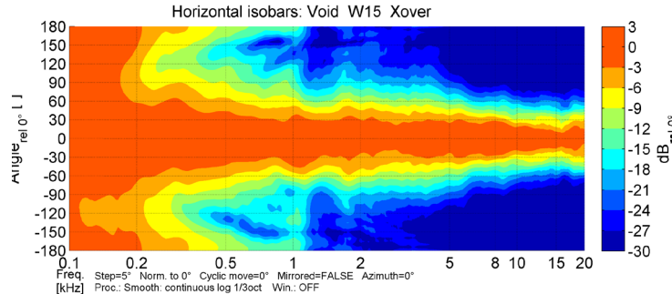
Figure 4.1: Horizontal directivity isobars
