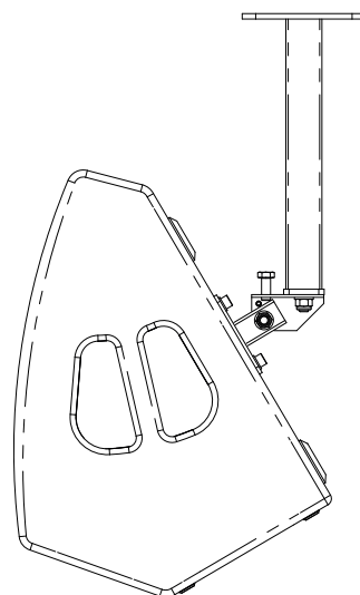
Figure 7.9: Alternative mounting orientation
