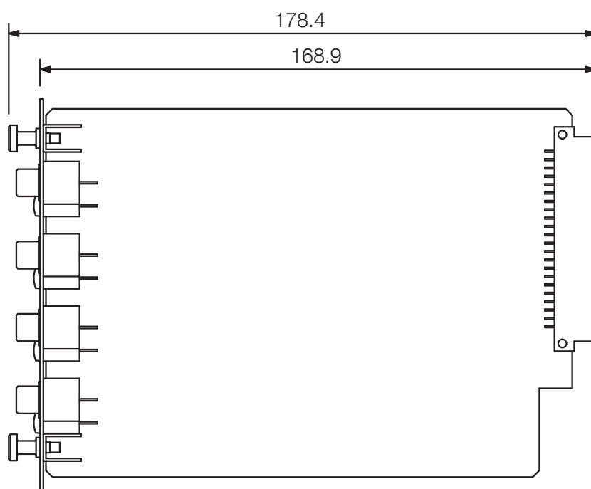
Side View
