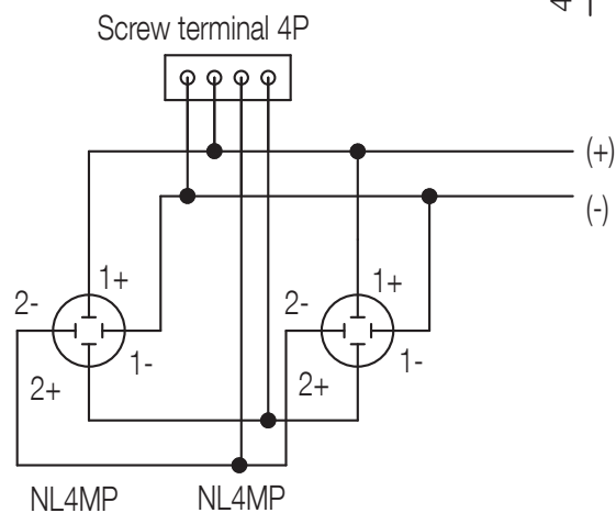
Wiring Diagram
