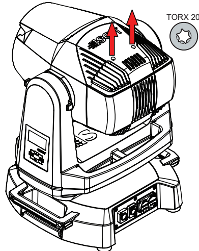
Figure 17: Removing the head cover
