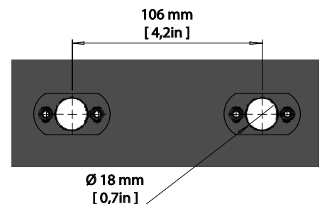
Figure 2: SGM locking points
