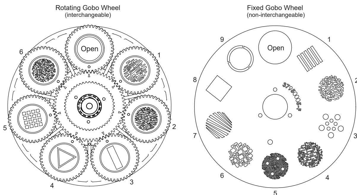
Figure 15: Identification of gobo wheels
