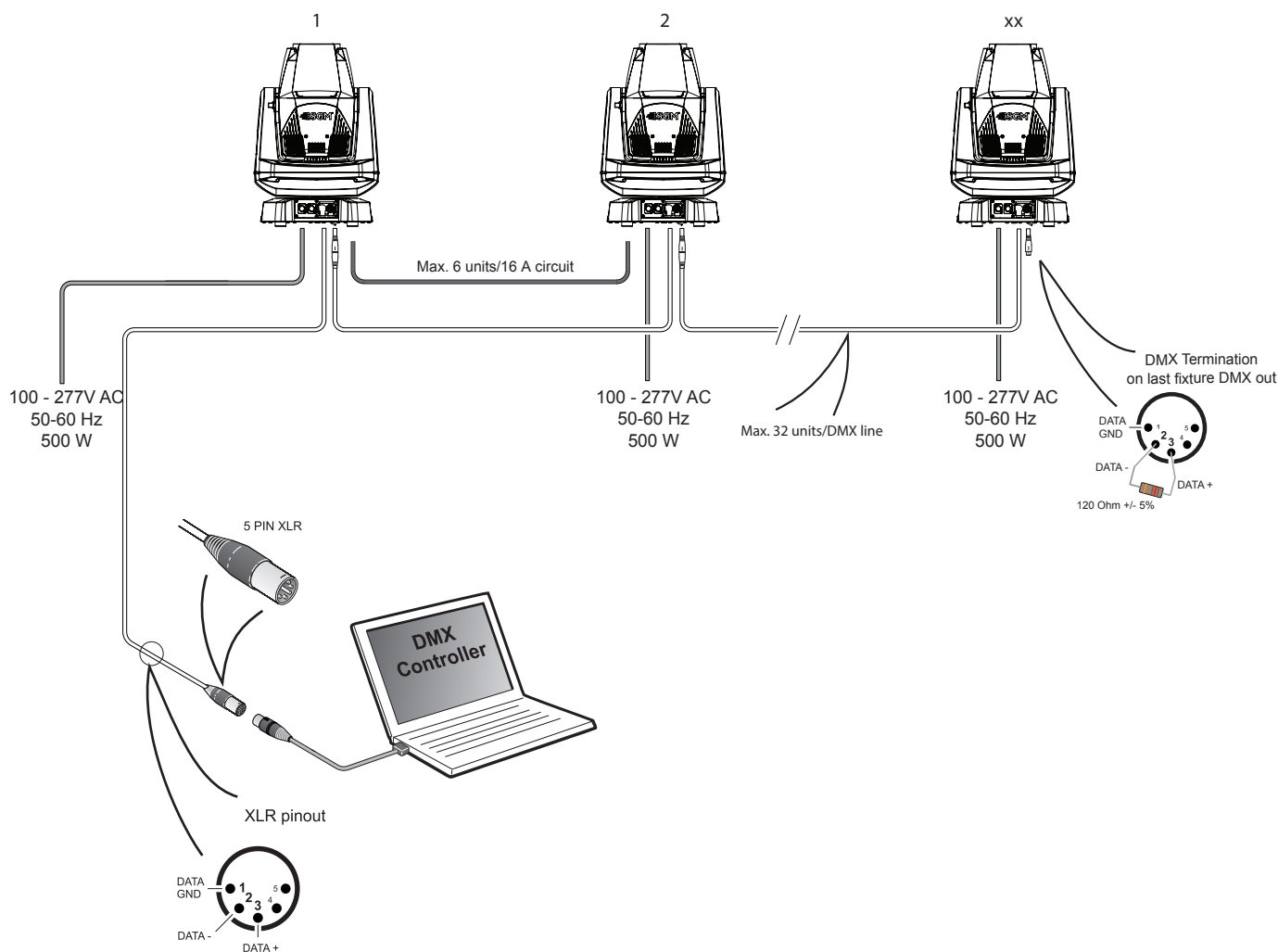
Figure 9: Connecting DMX in G-7 Spot
