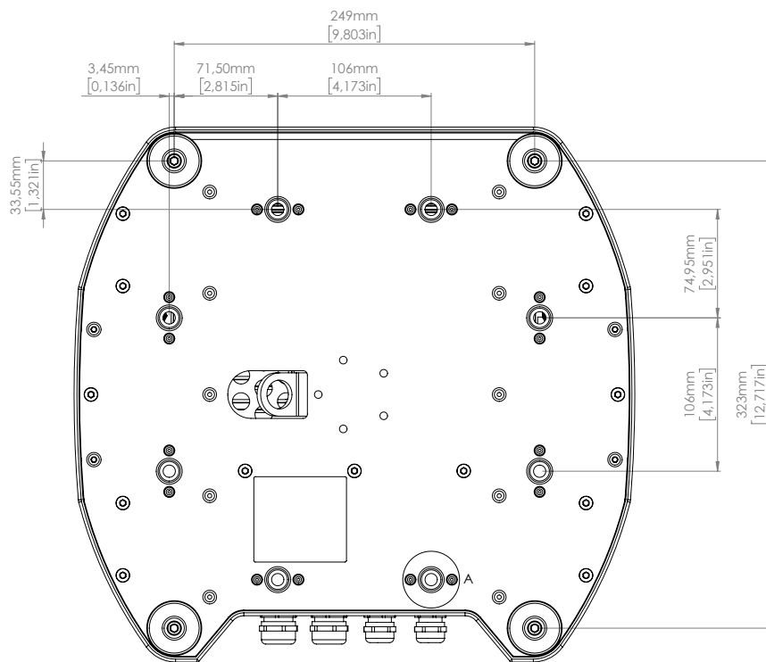
Figure 27: G-7 Spot base with dimensions
