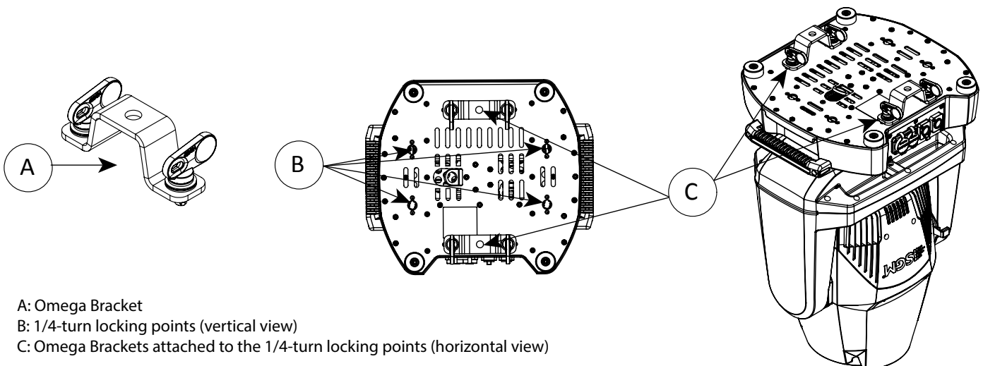
Figure 3: G-7 Spot base with Omega brackets
