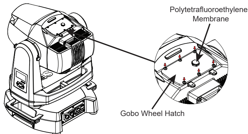
Figure 18: Removing gobo wheel hatch
