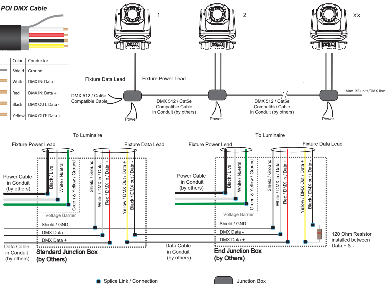
Figure 29: Connecting DMX and AC Power in G-7 Spot POI
