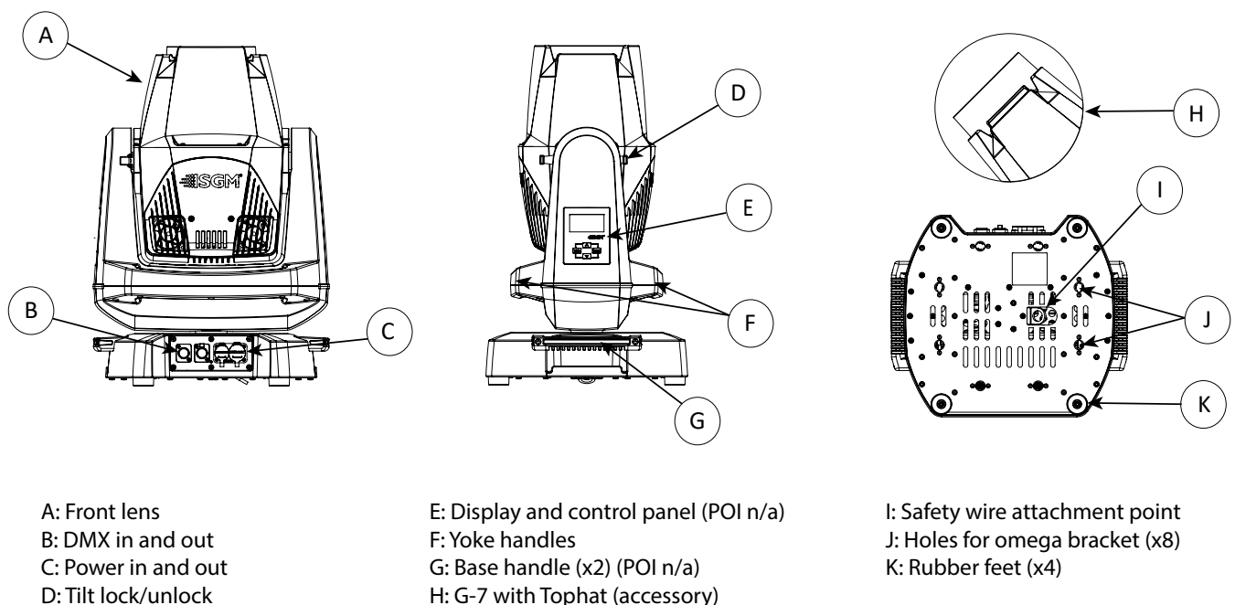
Figure 1: G-7 Spot parts and terminology
