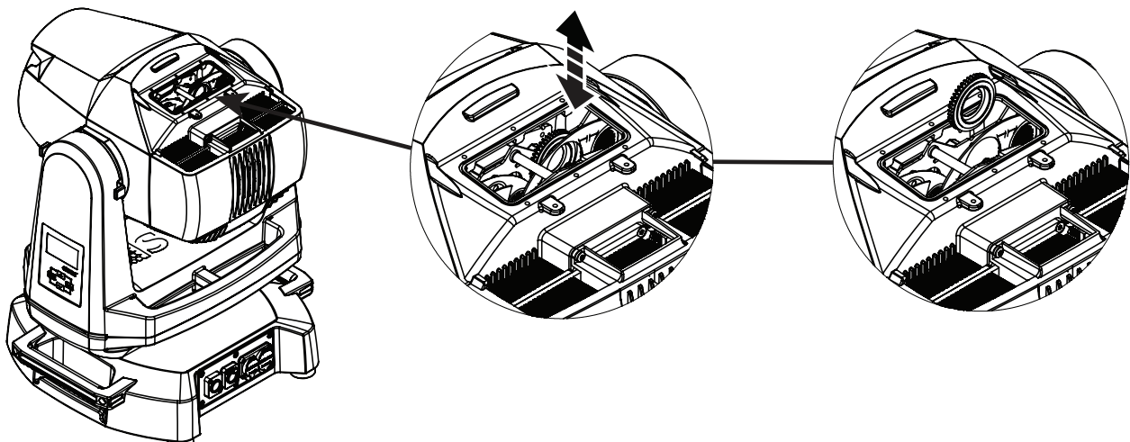
Figure 19: Removing gobo holder
