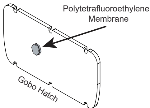
Figure 21: Polytetrafluoroethylene Membrane
