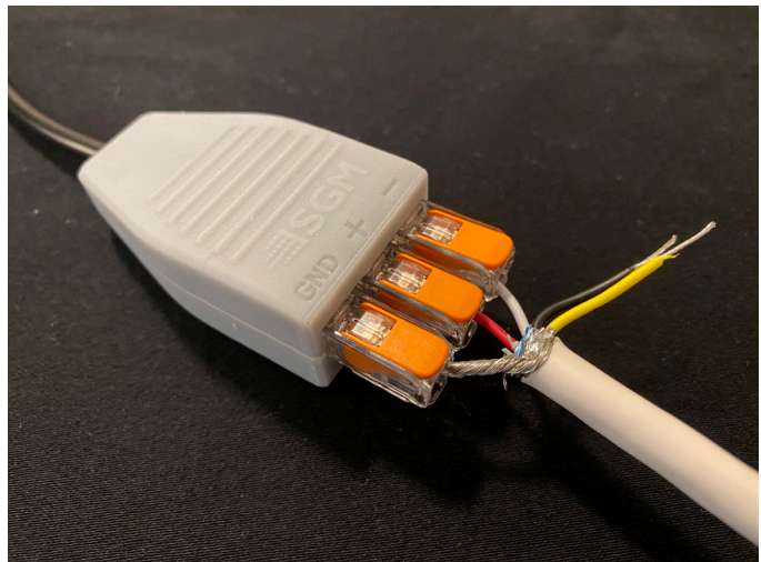
Figure 25: Connecting data to USB up-loader cable for POI fixtures
