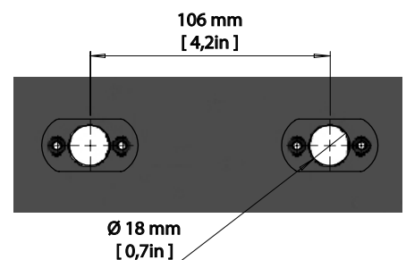
Figure 1: i-2 Series locking points
