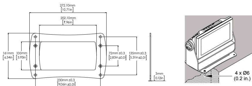
Figure 5: i-2 mounting bracket
