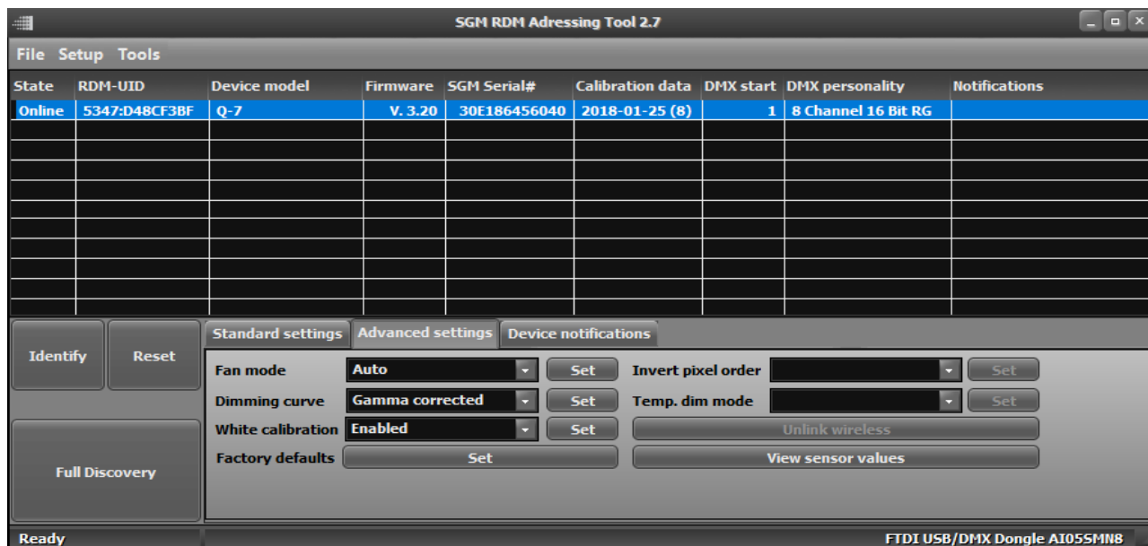
Figure 14: SGM Addressing tool
