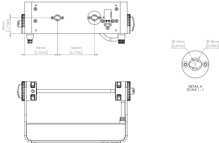
Figure 2: Dimensions for i-2 base locking points
