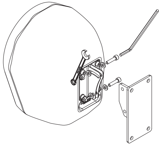
Figure 8.15: Mounting the loudspeaker
