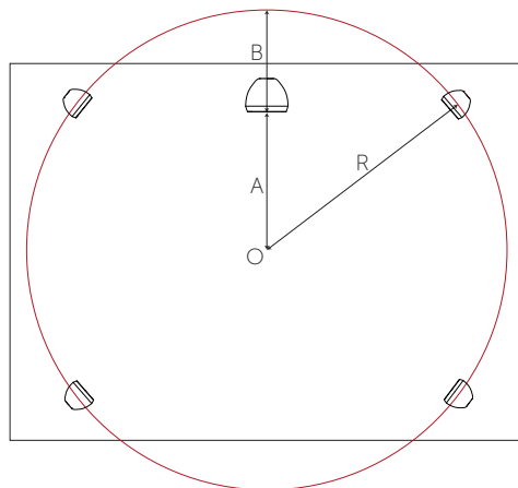
Figure 7.12: Bass alignment example 1
