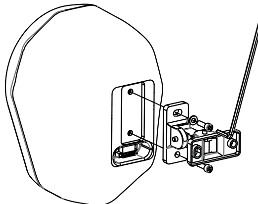
Figure 8.3: Bracket fixing
