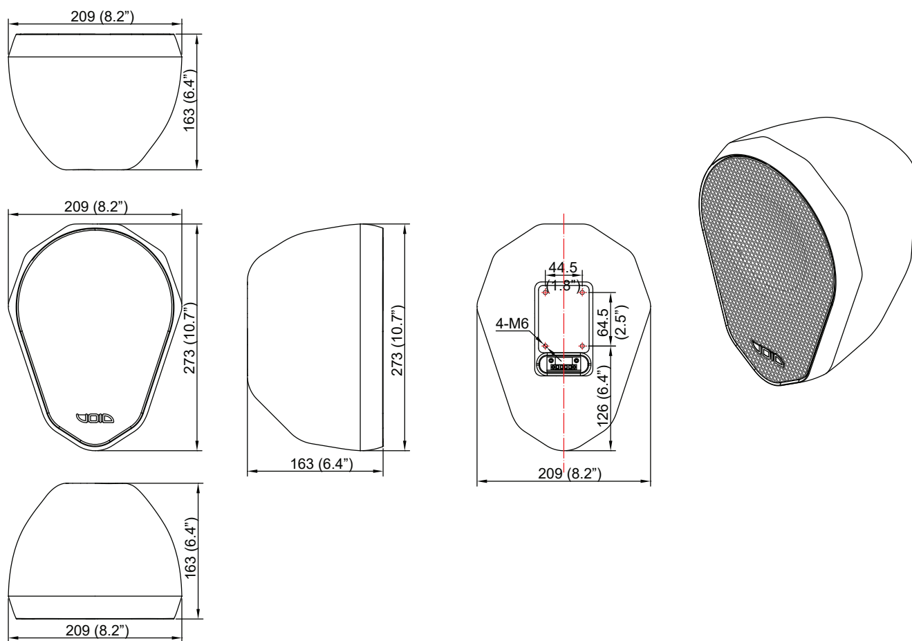
Figure 5.6: Dimensions
