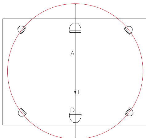
Figure 7.13: Bass alignment example 2
