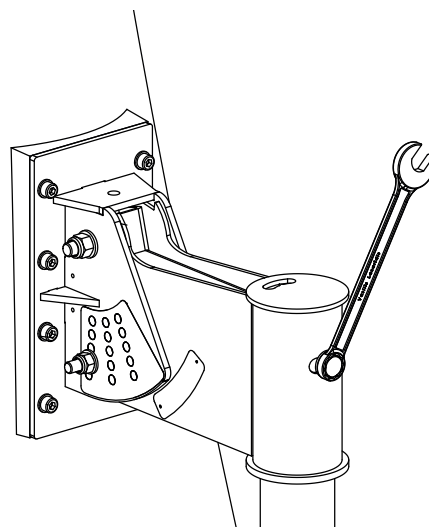
Figure 7.10: Securing the horizontal angle
