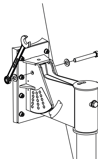
Figure 7.5: M12 bolt attachment
