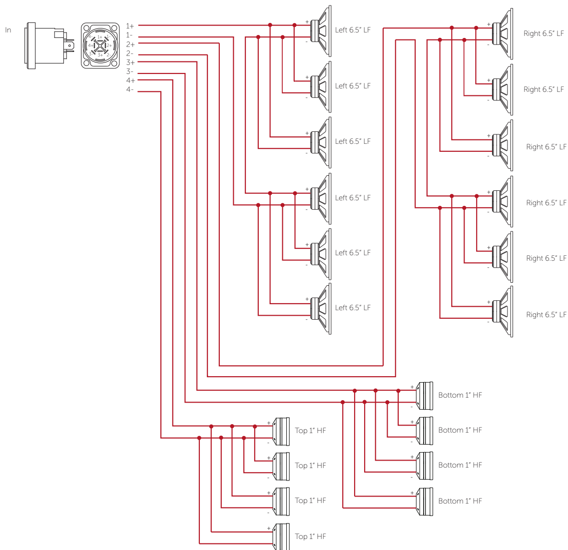
Figure 5.1: Wiring diagram
