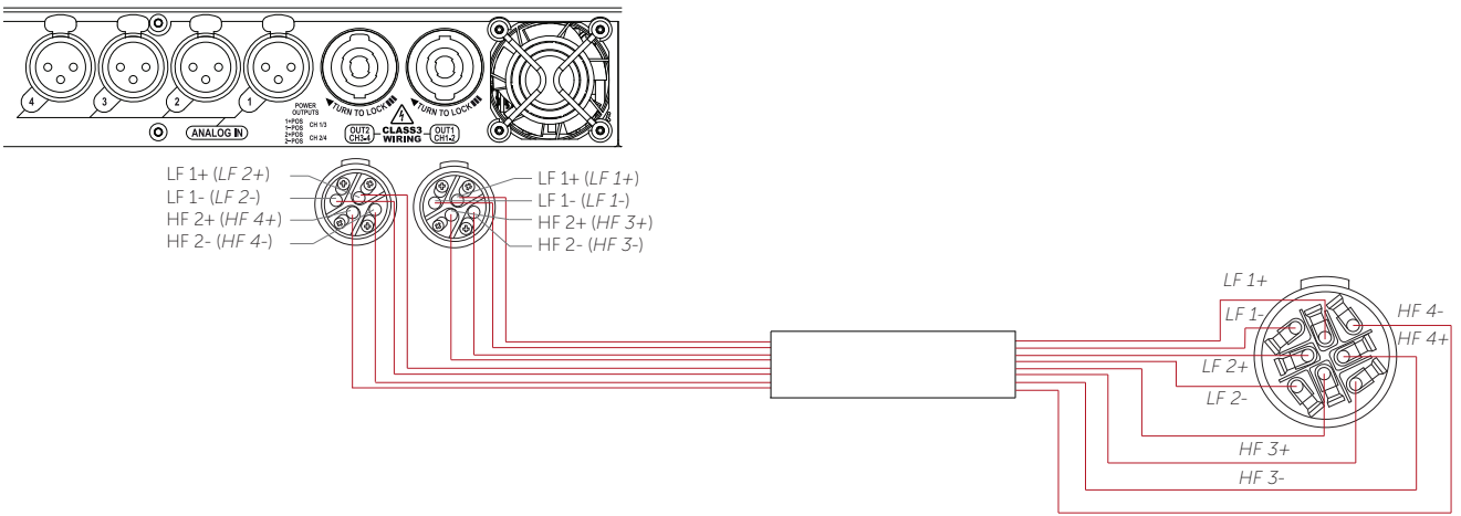
Figure 5.2: Bias Q5
