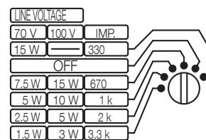
Impedance selection
