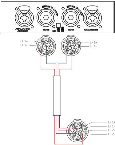
Figure 5.3: Bias V9
