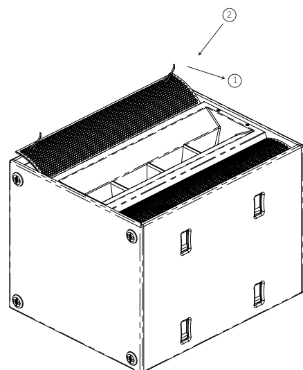
Figure 7.3: Grille replacement
