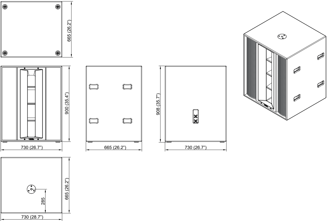
Figure 4.1: Dimensions
