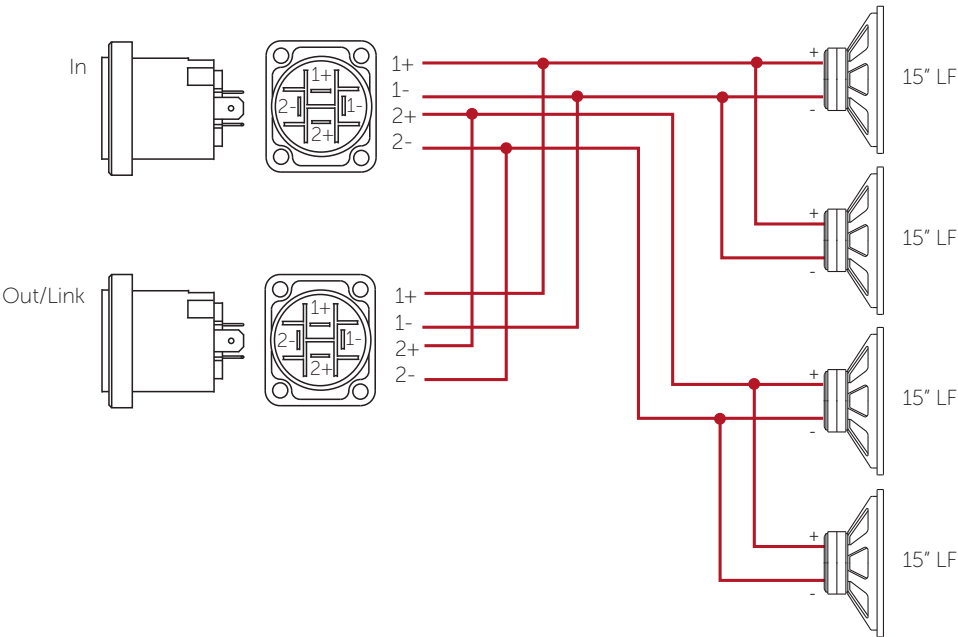
Figure 5.1: Wiring diagram
