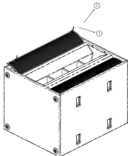
Figure 7.2: Grill removal
