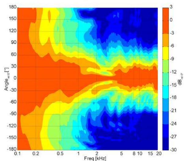
Figure A.12: Vertical directivity isobars
