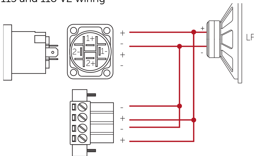
Figure 4.3: Single low frequency loudspeaker wiring diagram
