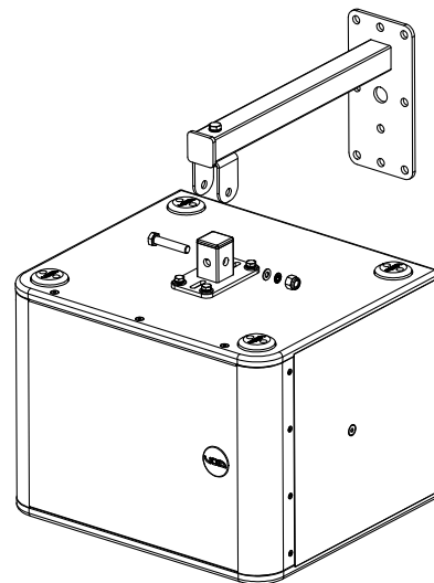
Figure 5.40: Loudspeaker fixing
