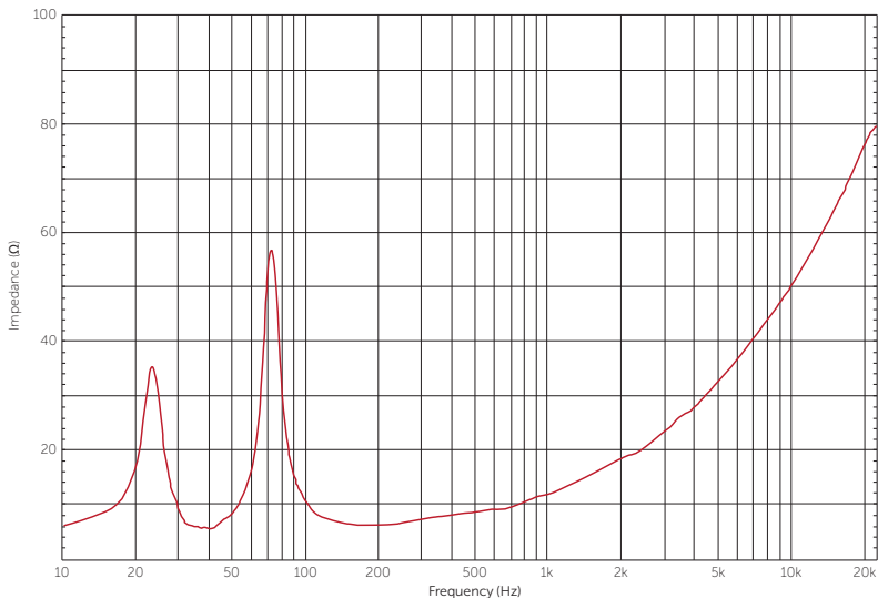
Figure A.15: Venu 115 V2 impedance graph
