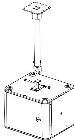
Figure 5.46: Loudspeaker fixing
