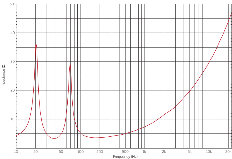
Figure A.17: Venu 215 impedance graph
