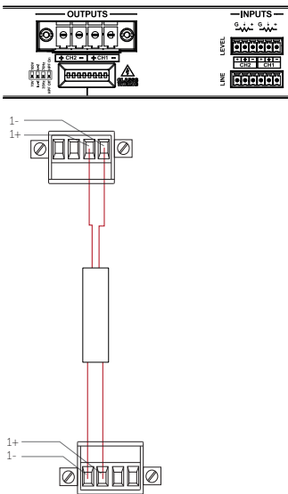
Figure 4.6: Bias D1 Phoenix wiring
