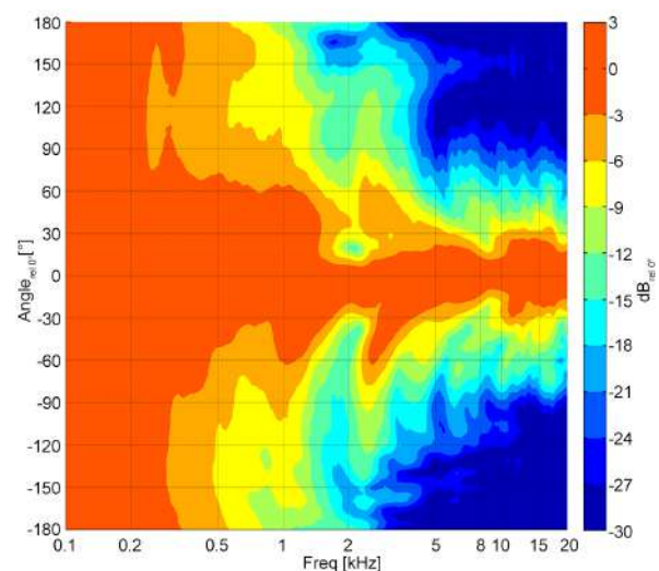
Figure A.2: Vertical directivity isobars
