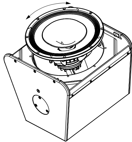
Figure 5.33: Rotating horn
