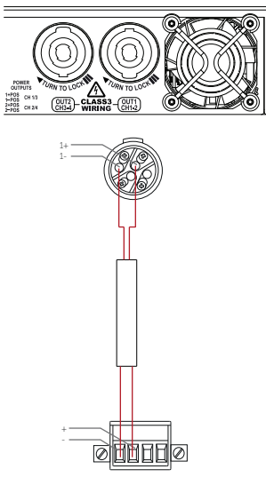
Figure 4.8: Bias Q3/Q5 speakON™ wiring
