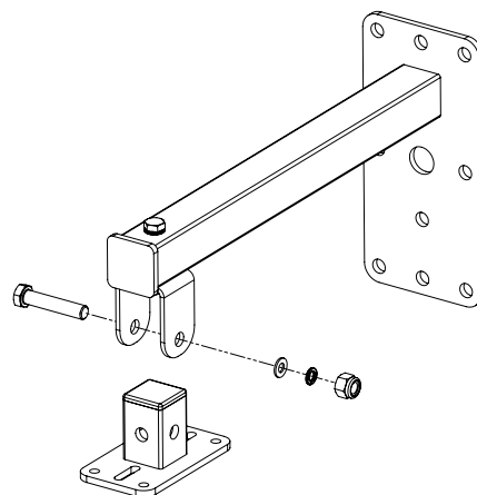
Figure 5.37: Nut removal
