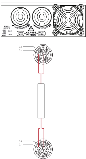
Figure 4.11: Bias Q3/Q5 speakON™ wiring
