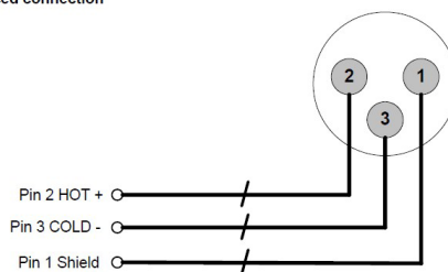
Input XLR balanced connection
