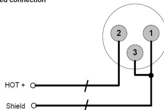
Input XLR unbalanced connection
