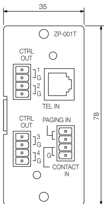
Front View
